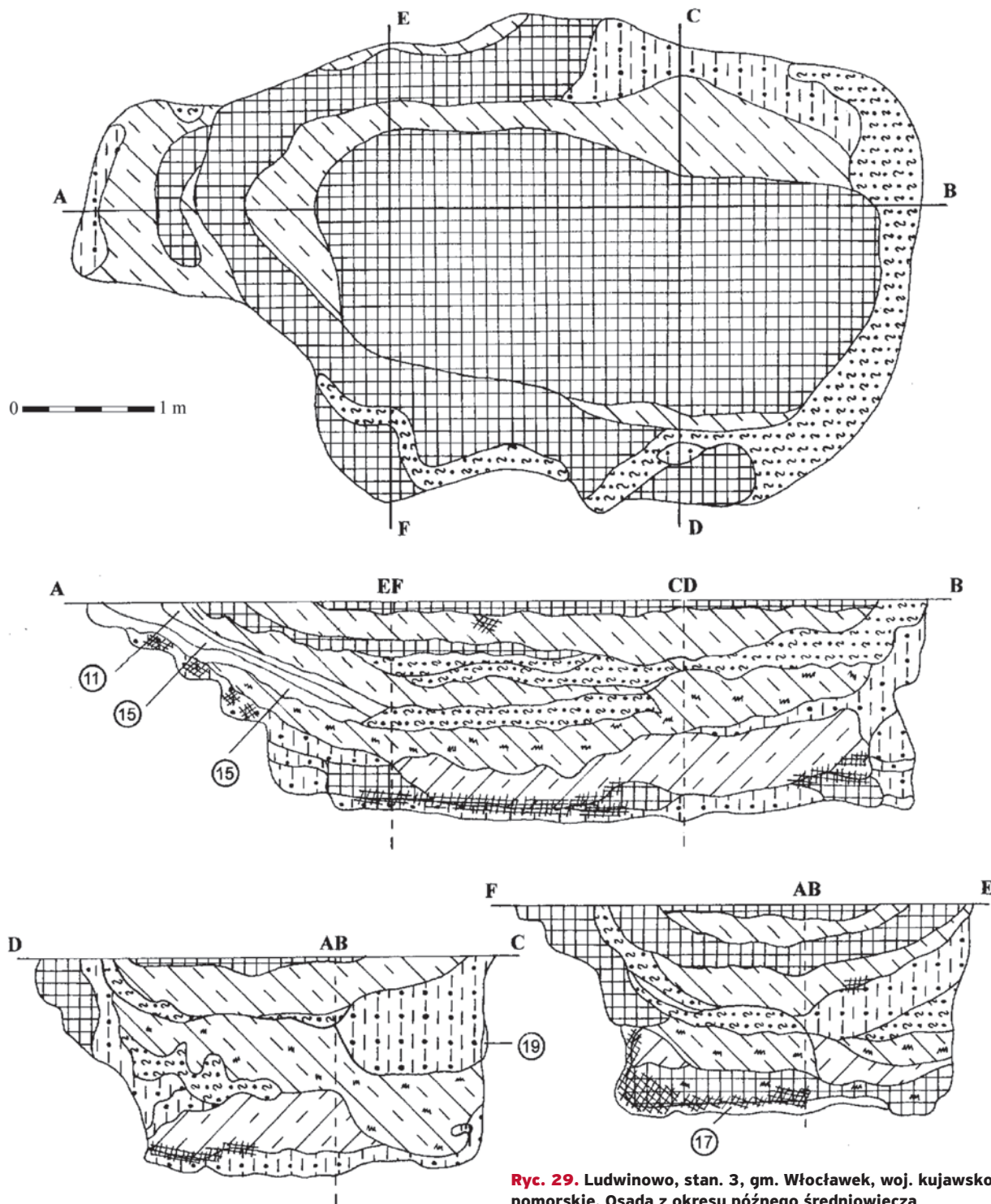
Ryc. 29. Ludwinowo, site 3, Włocławek commune, kujawsko-pomorskie voivodeship. Settlement from the period of the late Middle Ages and the early modern period. Object 434 – cellar remains (drawing by I. Nowak)
